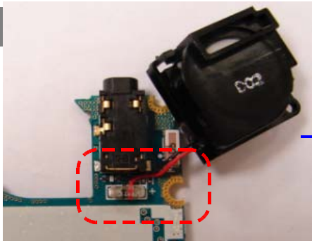
&lt;Assemble SPEAKER CONNECTOR&gt;
