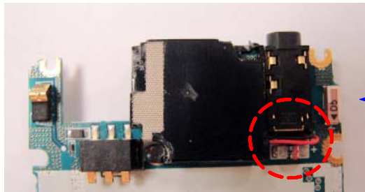
&lt;Push the SPK wires neatly&gt;
