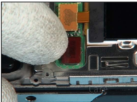
12. Close the LCD AM 240x320 flex connector.
